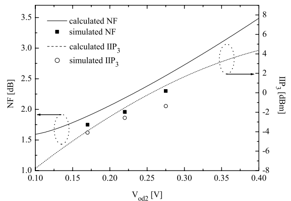
Fig. 9 Calculated and simulated NF and IIP 3 versus V_{od2} .
